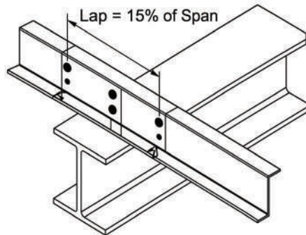
STRUCTURAL LAP
