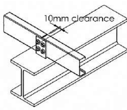
DOUBLE CLEAT
